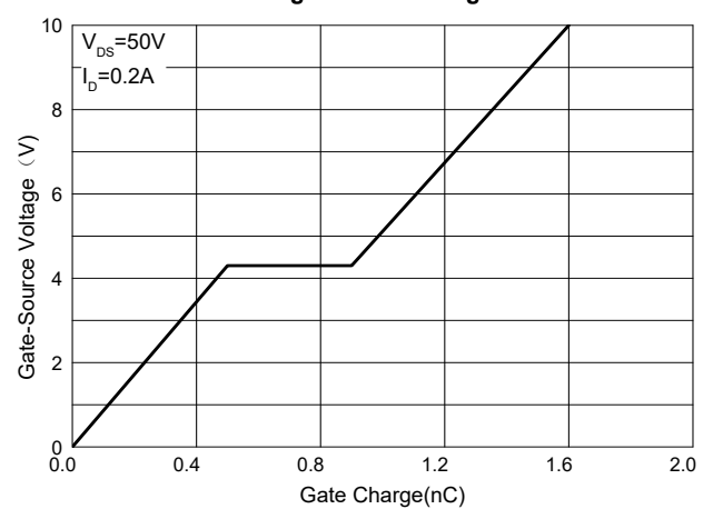
Fig.6 - Gate Charge
