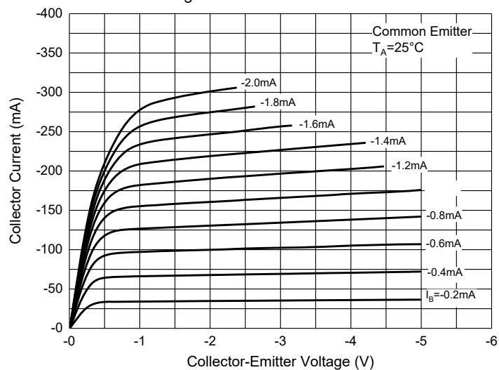
Fig. 1 - Static Characteristics
