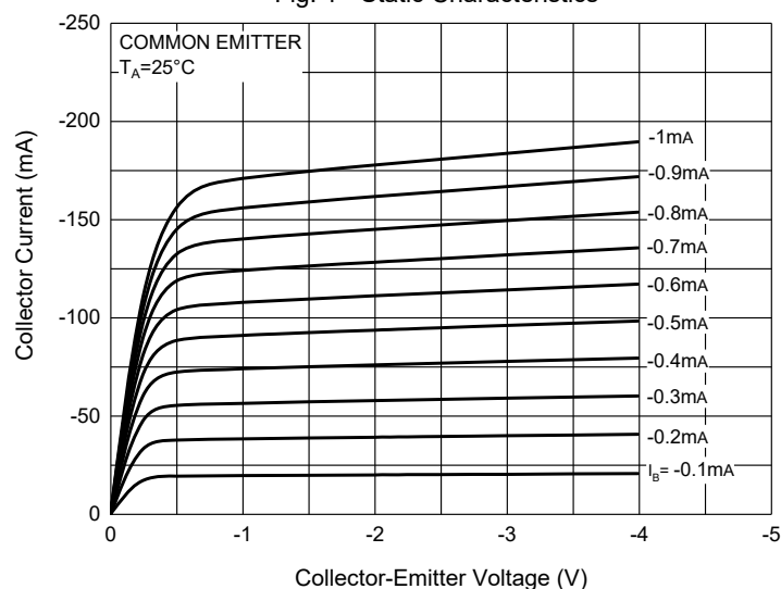
Fig. 1 - Static Characteristics
