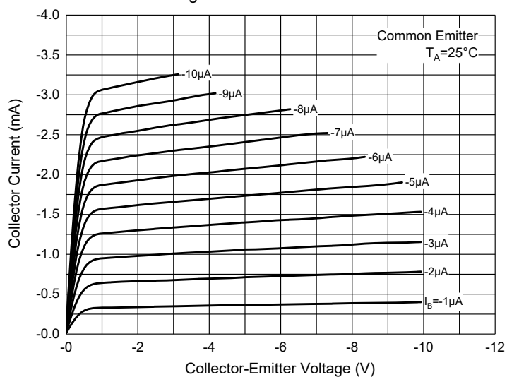
Fig. 7 - Static Characteristics
