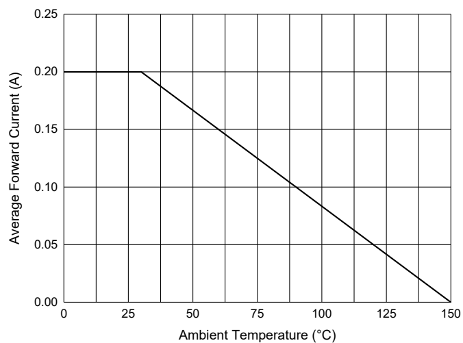
Fig. 4 - Current Derating Curve
