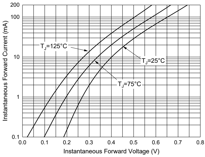
Fig. 1 - Forward Characteristics
