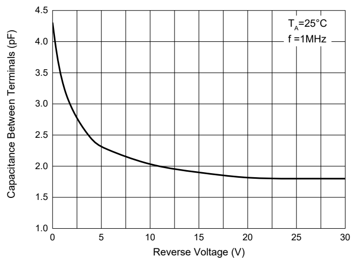
Fig. 3 - Capacitance Characteristics
