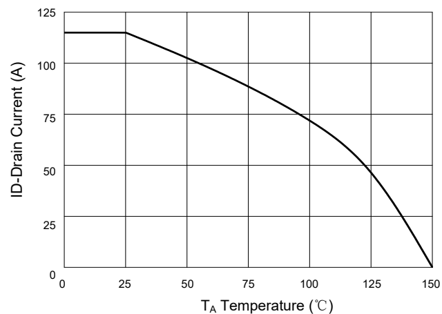
Fig.10 - Drain Current
