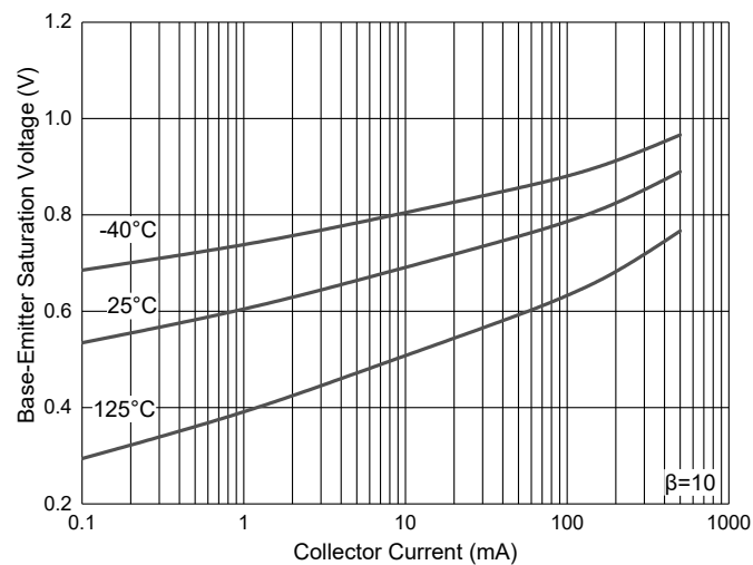
Fig. 6 - Base-Emitter Saturation Voltage Characteristics
