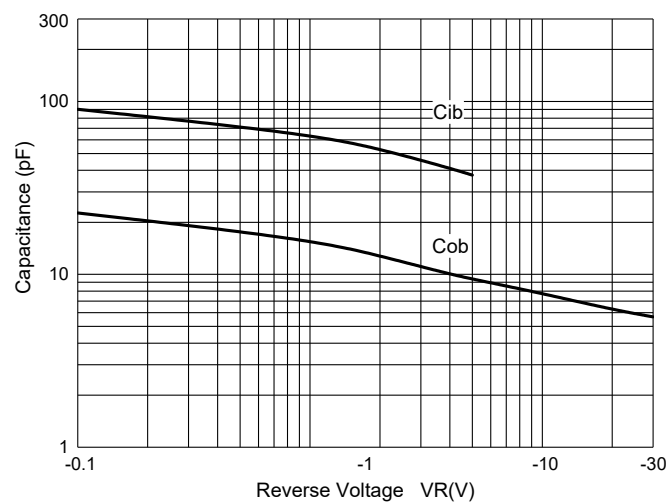
Fig. 7 - C_{ob}/C_{ib}—V_{CB}/V_{EB}
