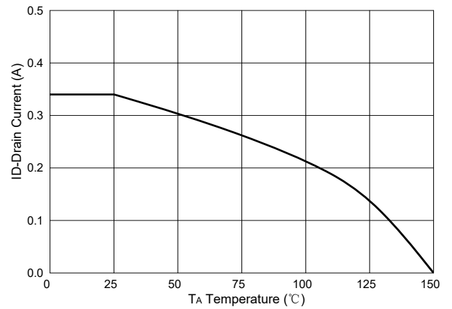
Fig. 10 - Drain Current
