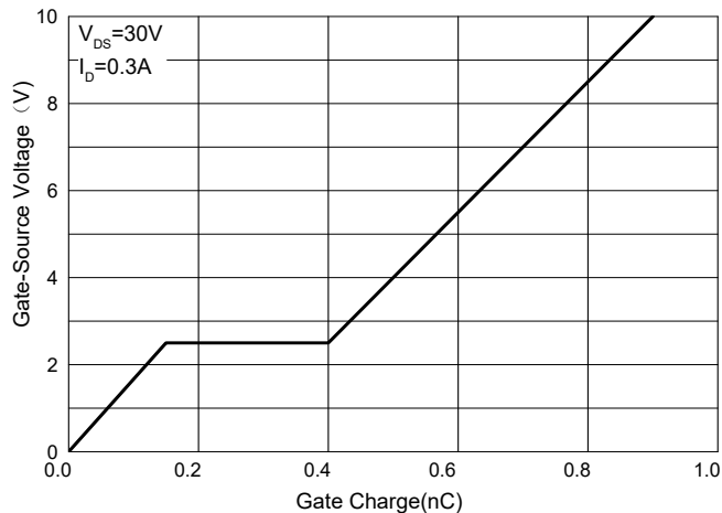
Fig.6 - Gate Charge
