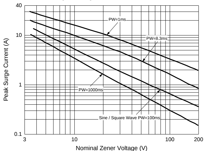
Fig. 5 - Surge Current Characteristics
