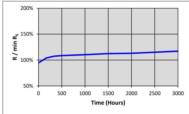
Figure 4: Accelerated Aging ESR Performance
