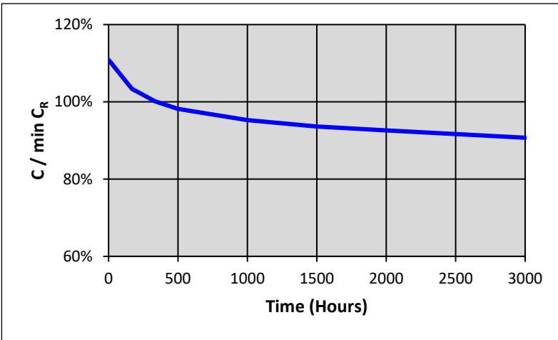
Figure 3: Accelerated Aging Capacitance Performance
