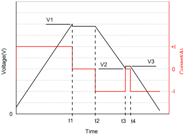
Figure 2: Cycle Life Test Waveform
