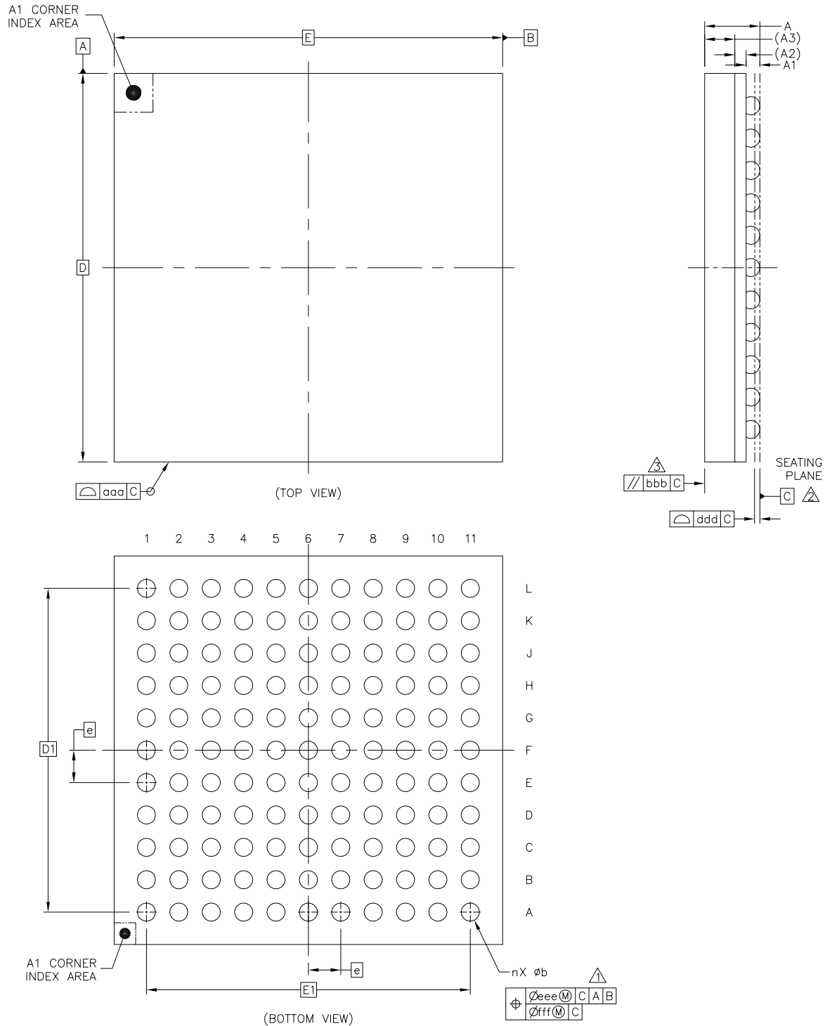
Figure 51: TMC8462-BA package outline drawing
