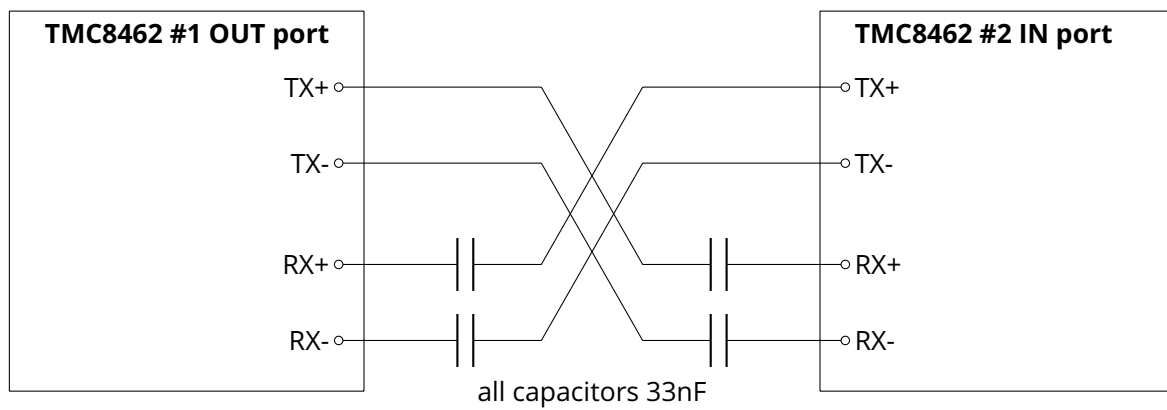
Figure 29: Direct PHY to PHY connection
