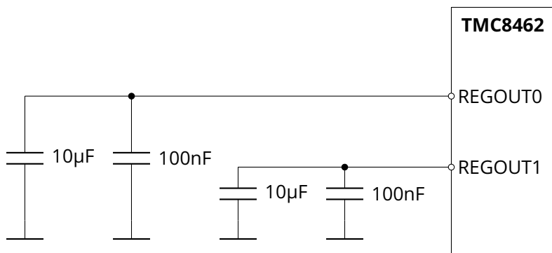
Figure 19: PHY power regulator filtering
