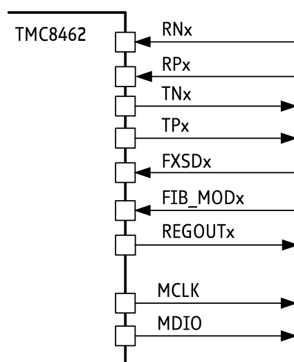
Figure 17: Physical bus interface pins
