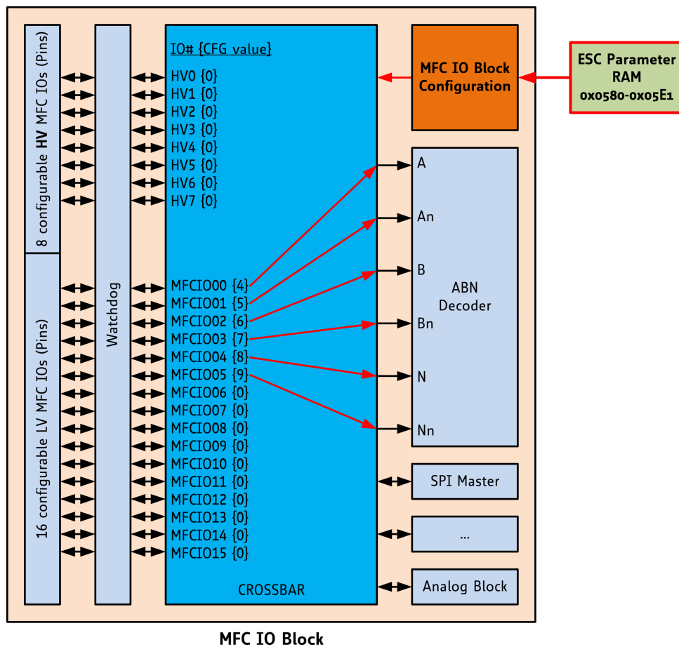
Figure 31: MFC IO Crossbar Example Configuration
