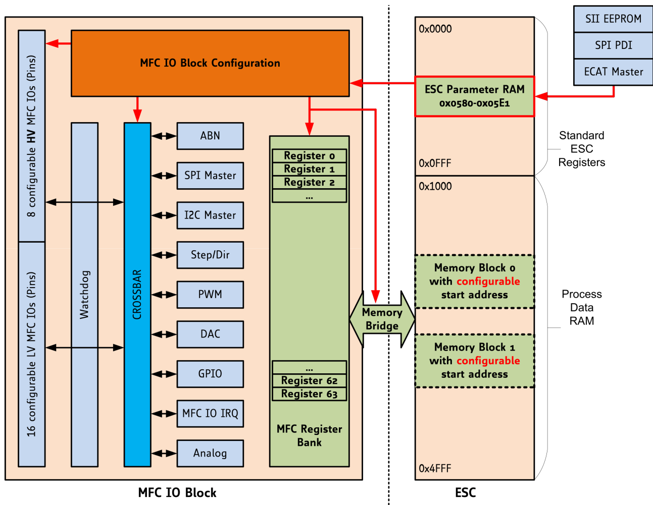
Figure 30: MFC IO Block Configuration using the ESC Parameter RAM
