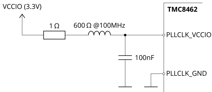
Figure 18: PLL supply filter
