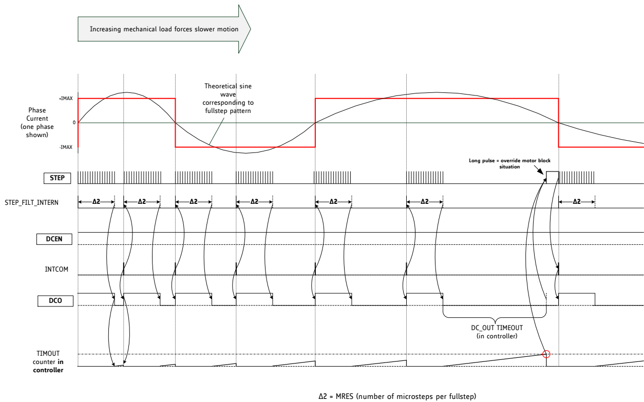
Figure 19.5 DCO Interface to motion controller – step generator stops when DC0 is asserted
