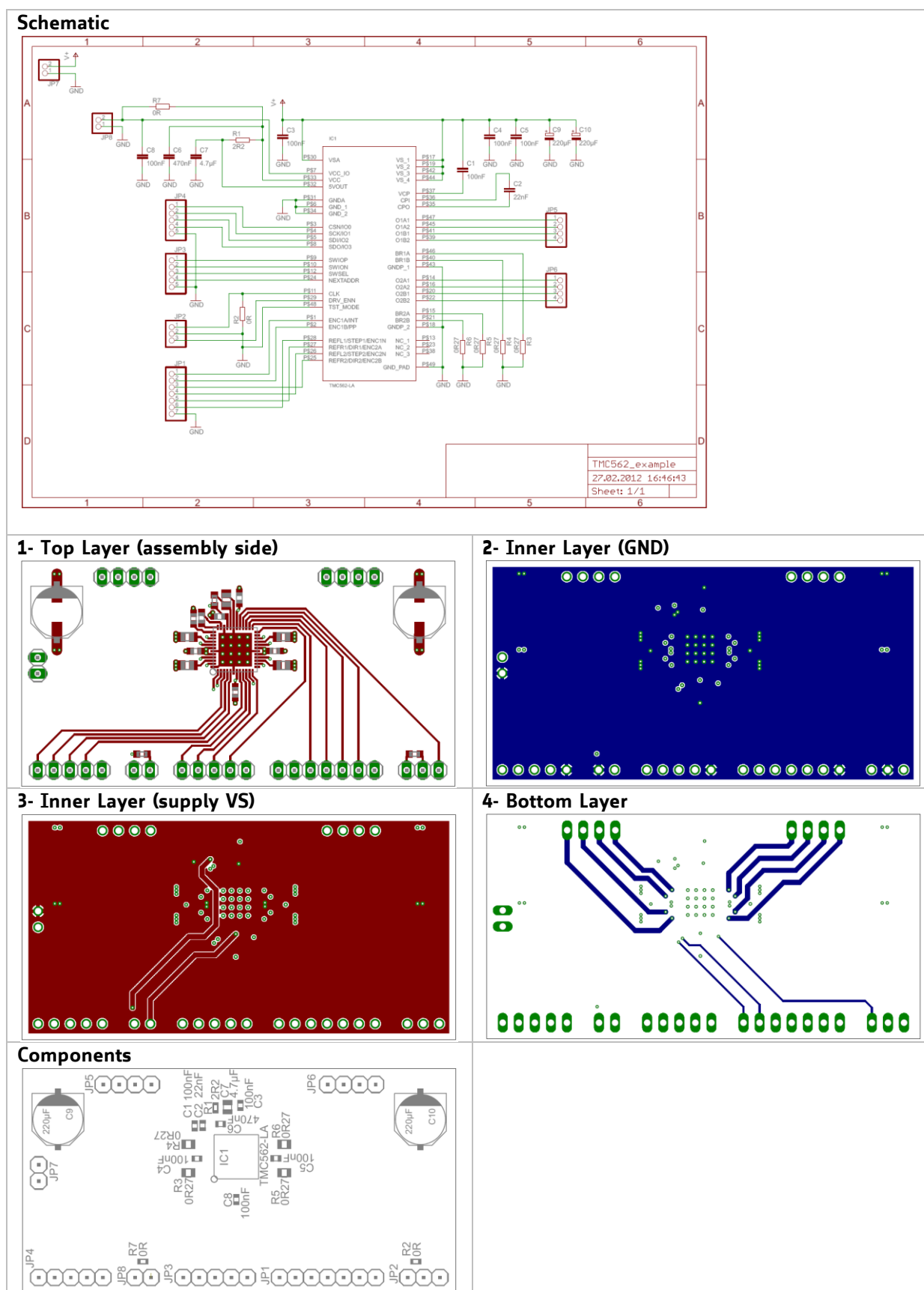
Figure 24.1 Layout example
