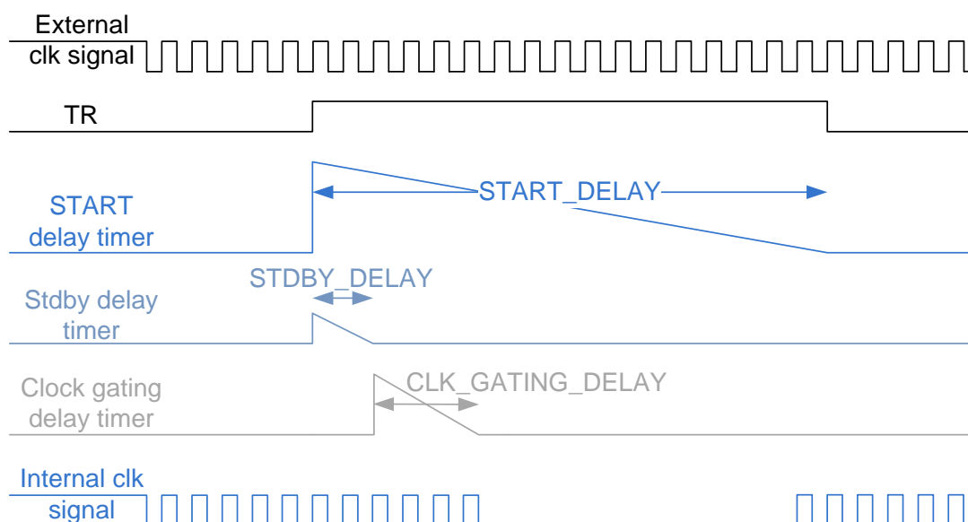
Figure 71: Automatic Clock Gating Activation and Wake-Up
