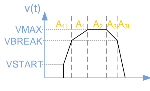
Figure 24: Trapezoidal Ramp with initial Velocity
