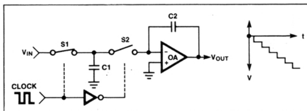
Figure 21. Simple Inverting Switched Capacitor Integrator
