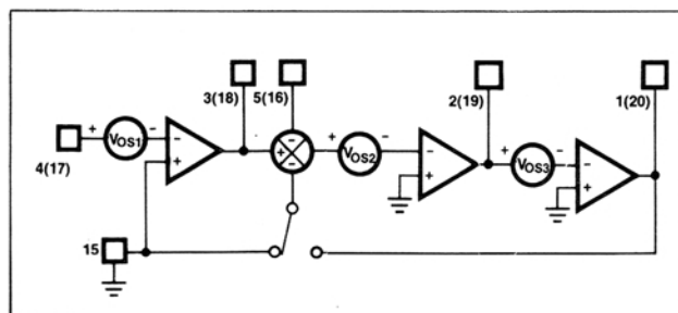
Figure 16. MF10 Offset Model
