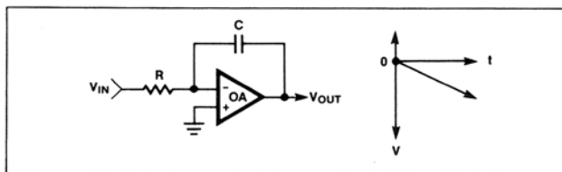
Figure 20. Typical RC integrator
