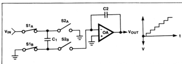
Figure 22. The Non-Inverting Integrator Used in the MF10
