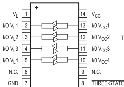
TSSOP-14 TOP VIEW
