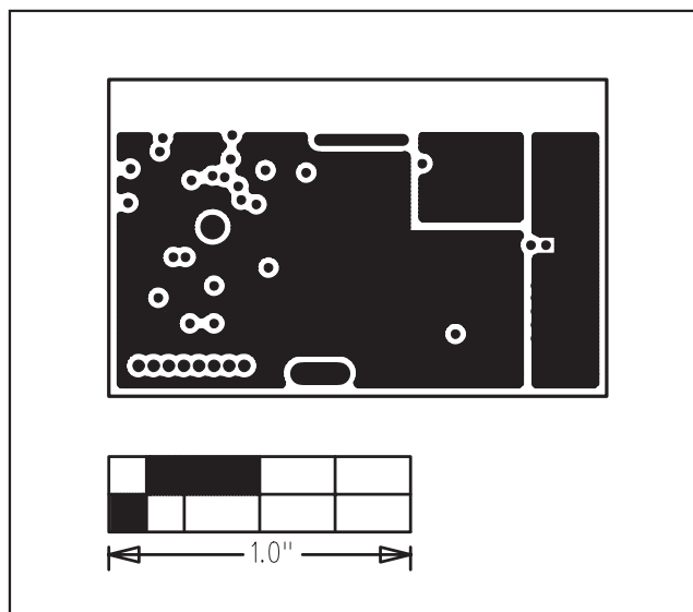
Figure 8. MAX5060 EV Kit PCB Layout—GND (Layer 5)
