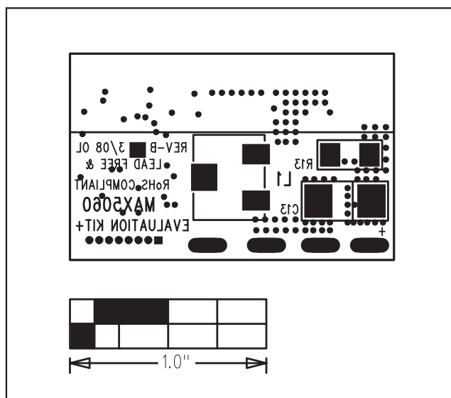
Figure 10. MAX5060 EV Kit Component Placement Guide—Bottom Layer
