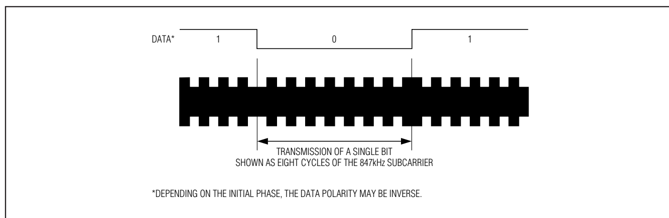
Figure 9. Uplink: Load Modulation of the RF Field by the BPSK Modulated Subcarrier
