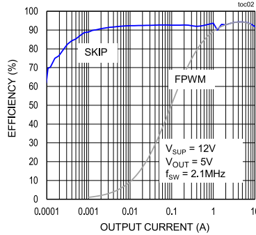
EFFICIENCY & POWER LOSS vs OUTPUT CURRENT ( V_{OUT} = 5\text{V} )
