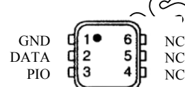
TOP VIEW 3.7 X 4.0 X 1.5
