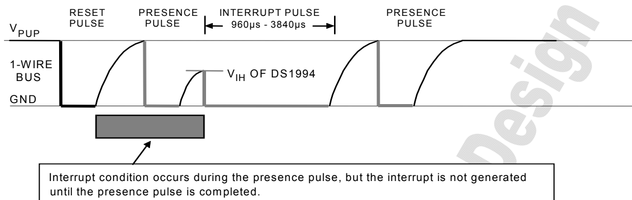
Figure 14. TYPE 2 INTERRUPT
