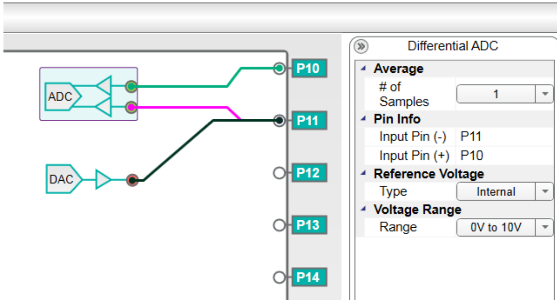
Figure 10. ADC with Pseudo-Differential Input Set by DAC
