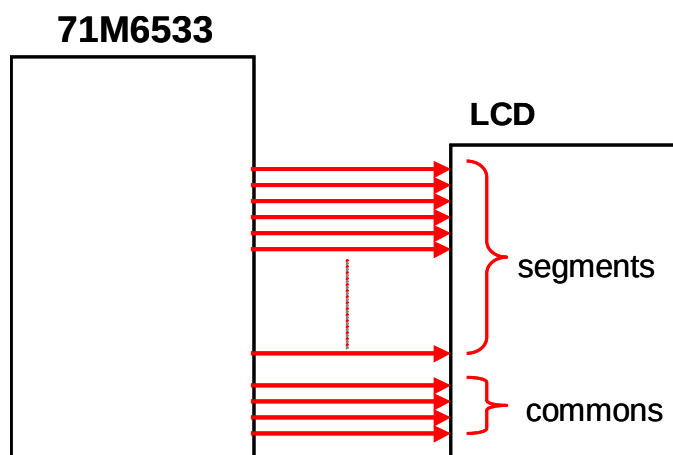
Figure 2-11: LCD Connections
