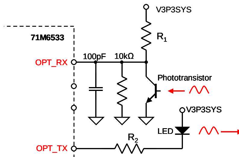
Figure 2-12: Optical Interface Block Diagram
