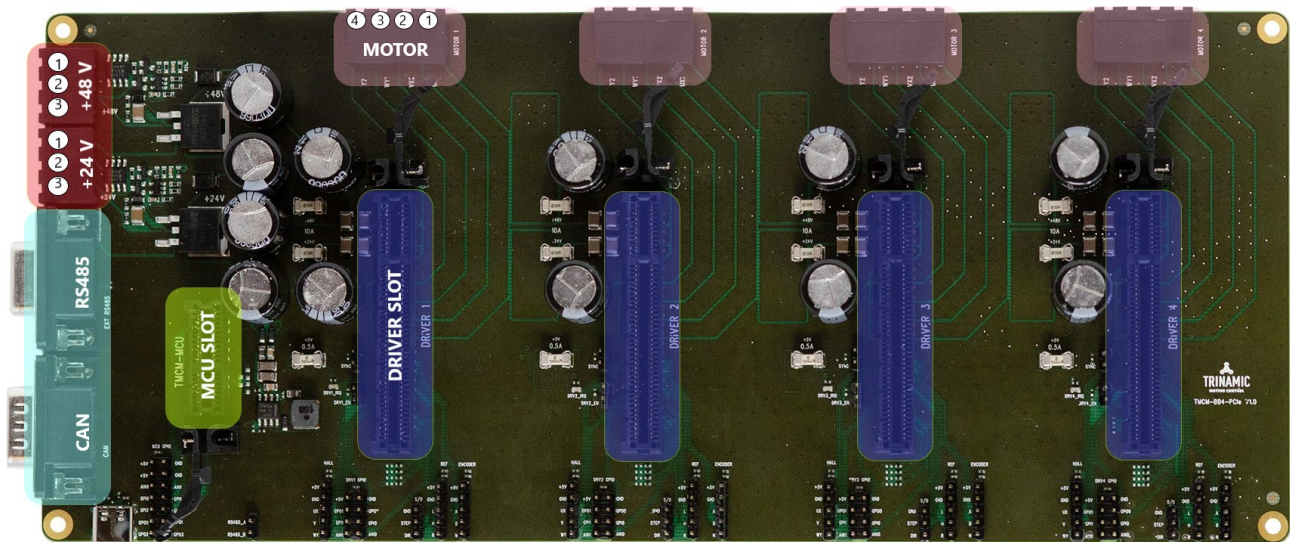
Figure 2: Top view of TMCB-BB4
