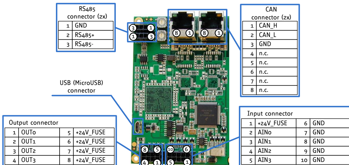
Figure 5.2 TMC6210 interface brick
