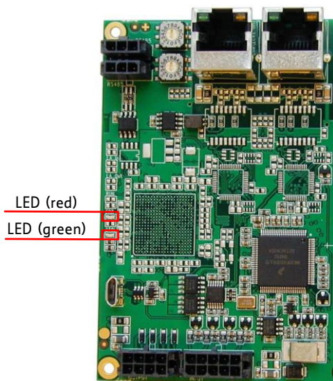
Figure 7.2: LEDs on TMC6210 interface brick
