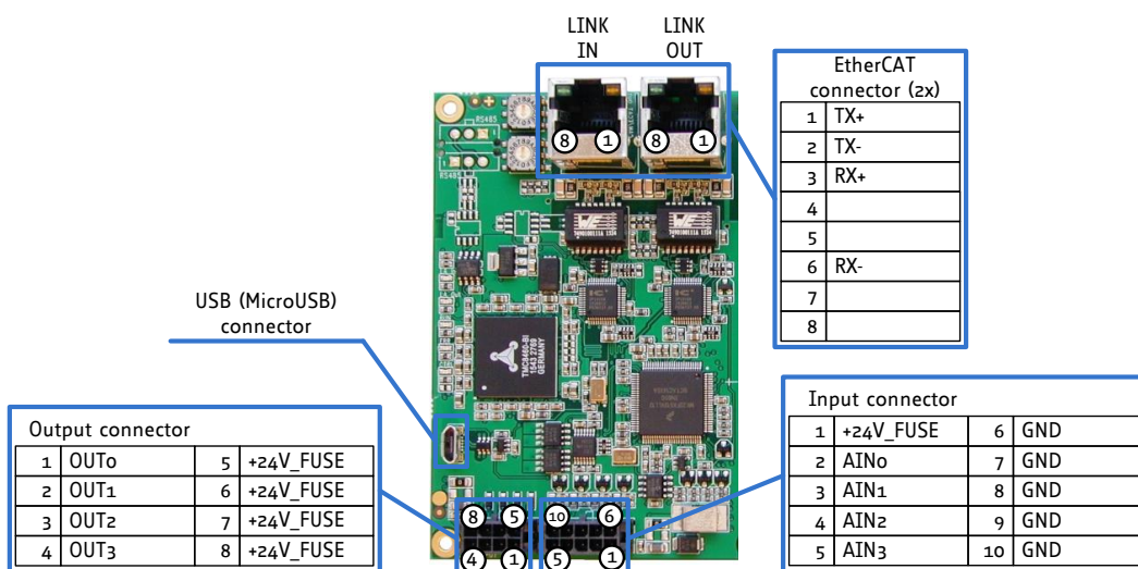
Figure 5.3 TMC-6211 interface brick
