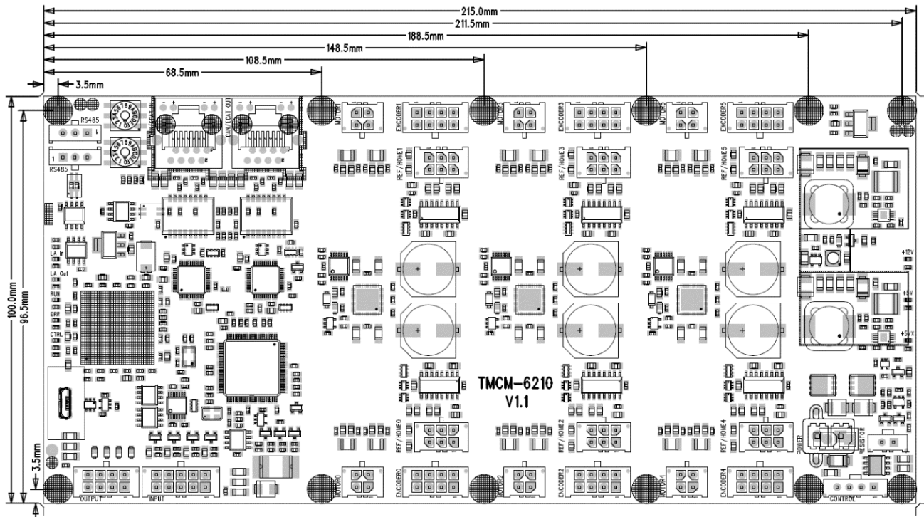
Figure 4.1 Dimension of TMC-6210 / TMC-6211 and position of mounting holes
