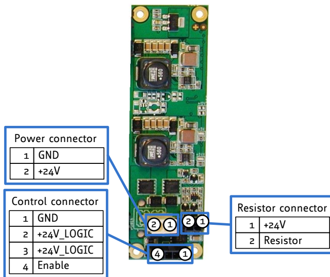
Figure 5.5: TMC6210 + TMC6211 Power supply Brick
