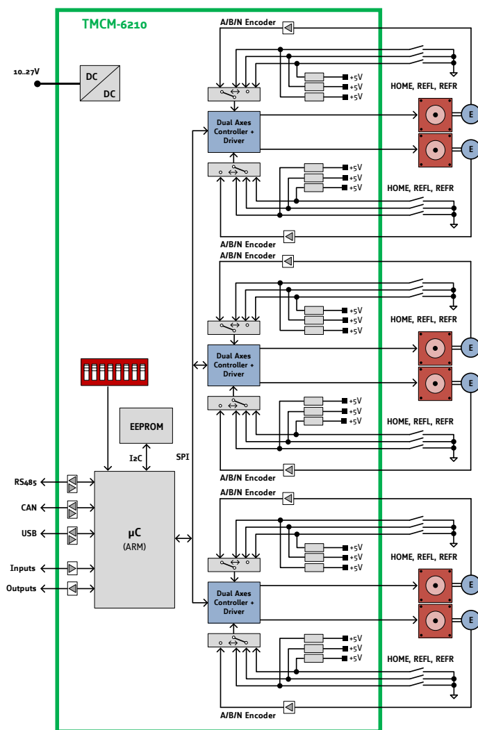
Figure 10.1 Main parts of the TMC6210
