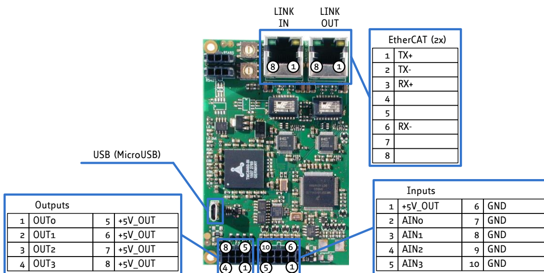
Figure 5.3 TMC-3215 interface brick
