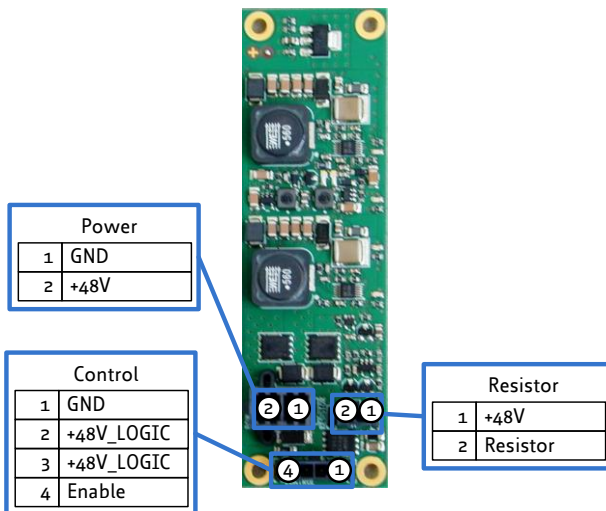
Figure 5.5: TMC3214 + TMC3215 Power supply Brick
