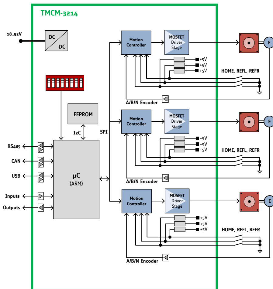
Figure 10.1 Main parts of the TMC3214
