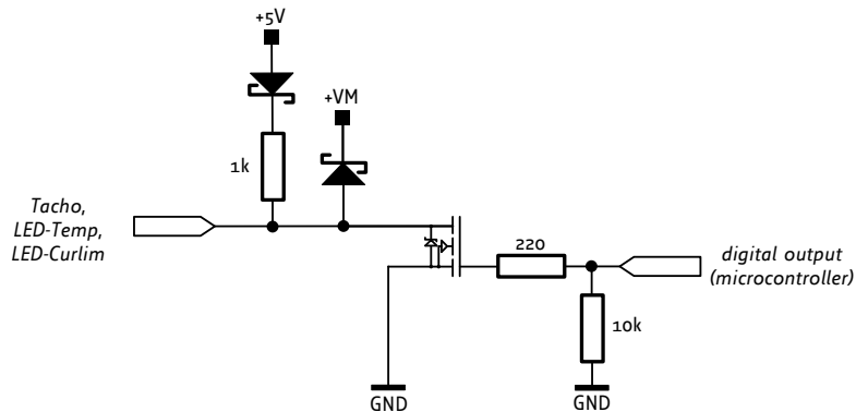
Figure 7: TCM-1633 output circuit (same circuit design for Tacho, LED-Temp and LED-CurLim outputs)
