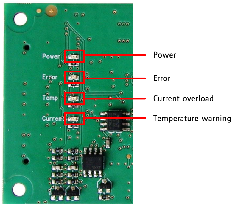
Figure 8: TMC-1633 LEDs
