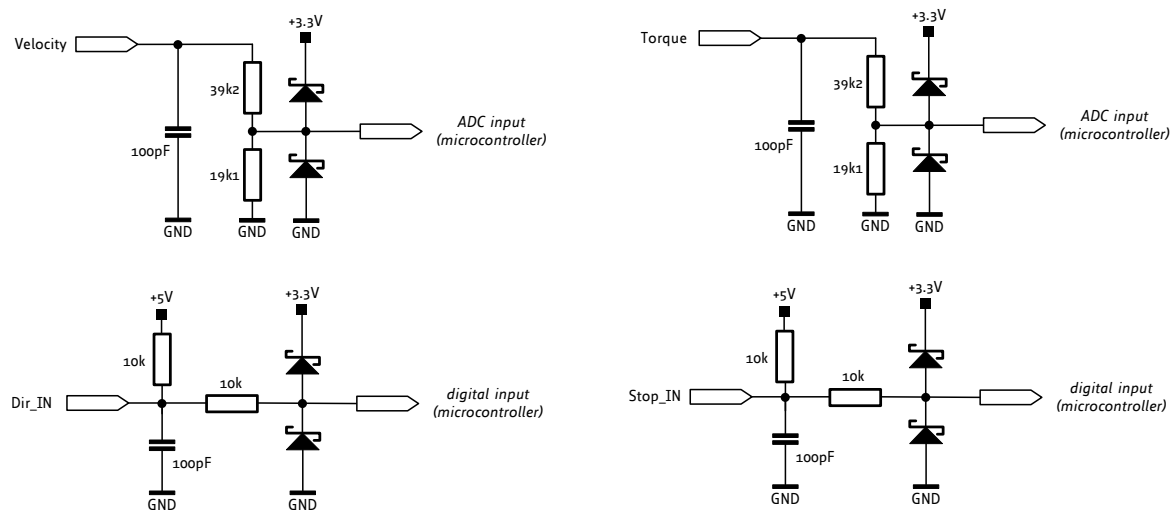
Figure 4: TMC-1633 input circuit for the general purpose analog and digital inputs
