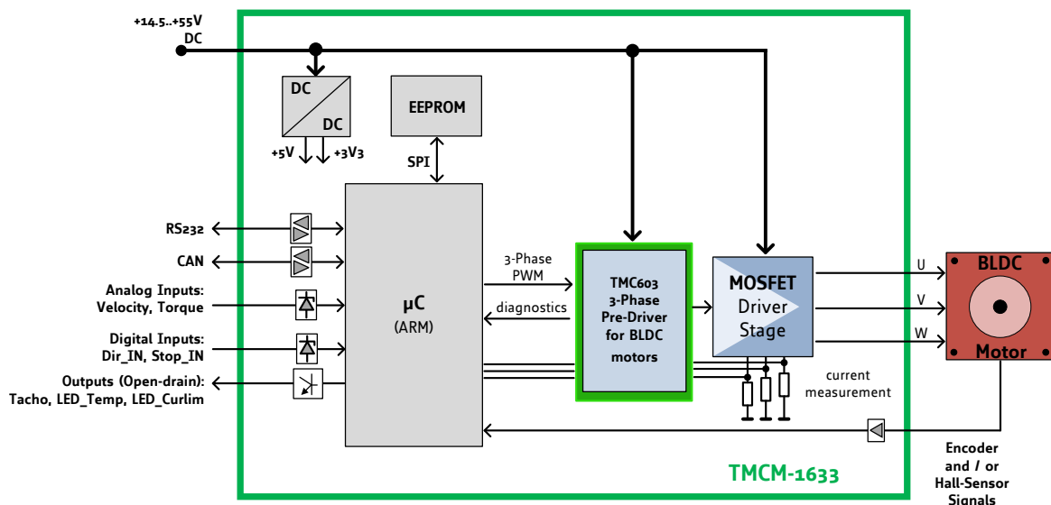
Figure 9: TMC-1633 block diagram
