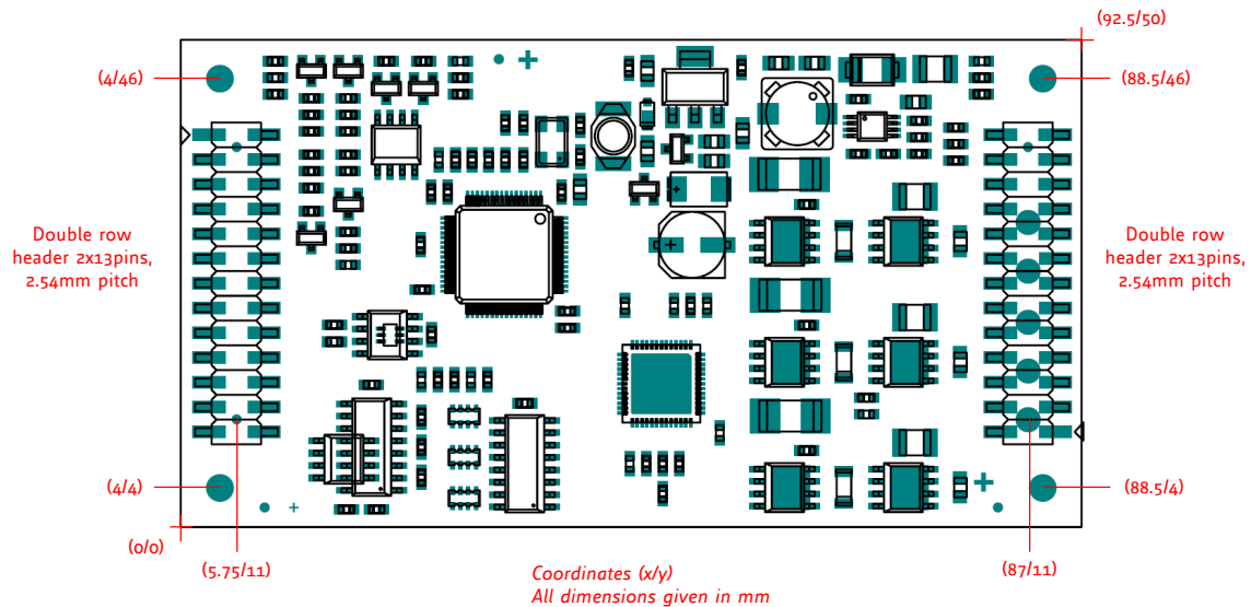
Figure 1: TCM-1633 mechanical dimensions
