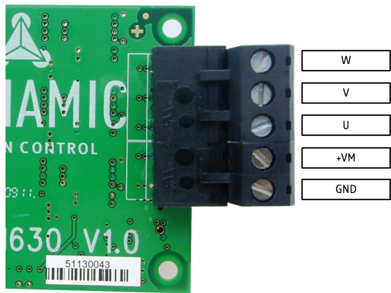
Figure 3: TMCM-1633 Connector
