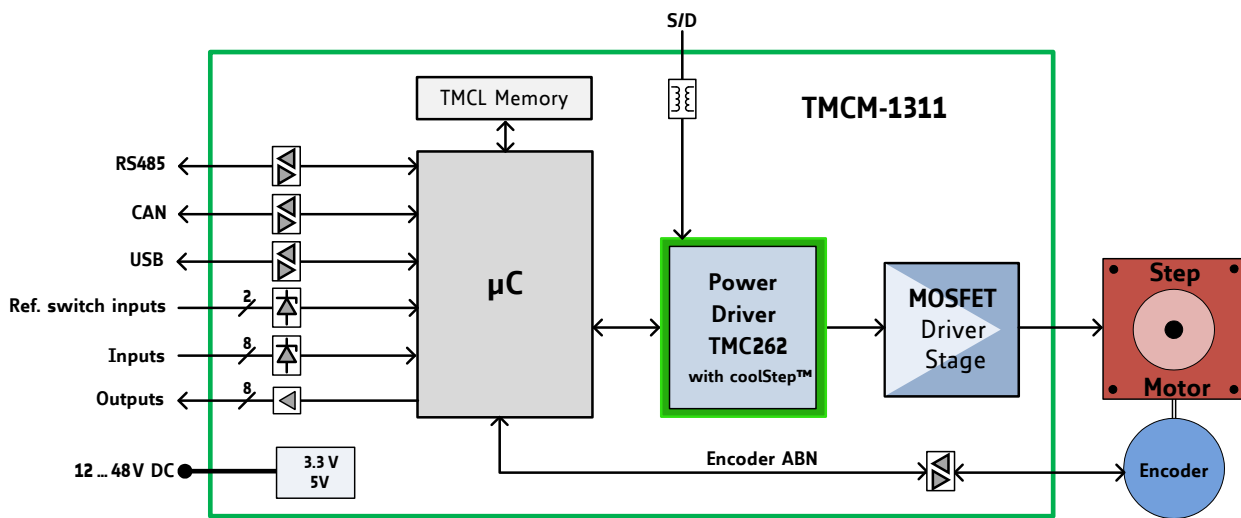
Figure 6.1 Main parts of TMC1311
