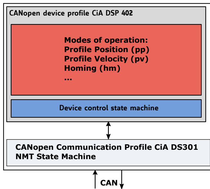
Figure 5: Communication Architecture
