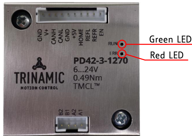
Figure 10: TCM-1270 LED colors and location
