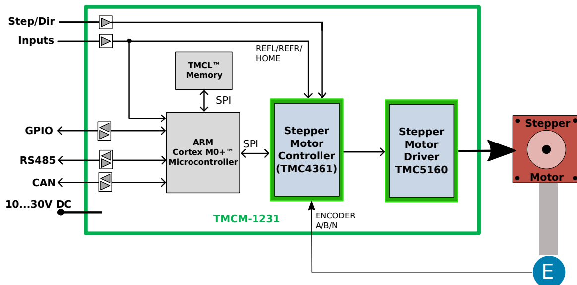
Figure 7: TMC-1231 block diagram
