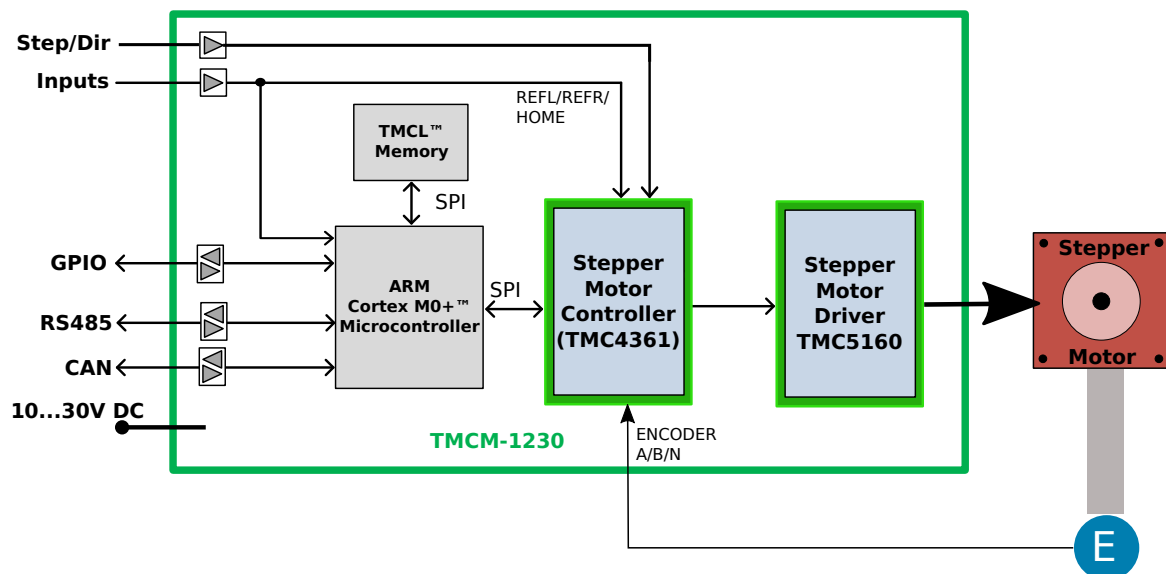
Figure 7: TMC-1230 block diagram
