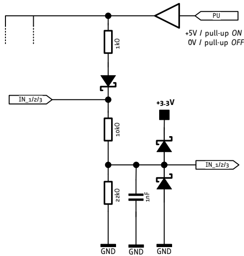
Figure 3.5 Internal circuit of IN_1/2/3
