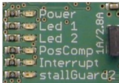
Figure 4: TMC-1111 LEDs
