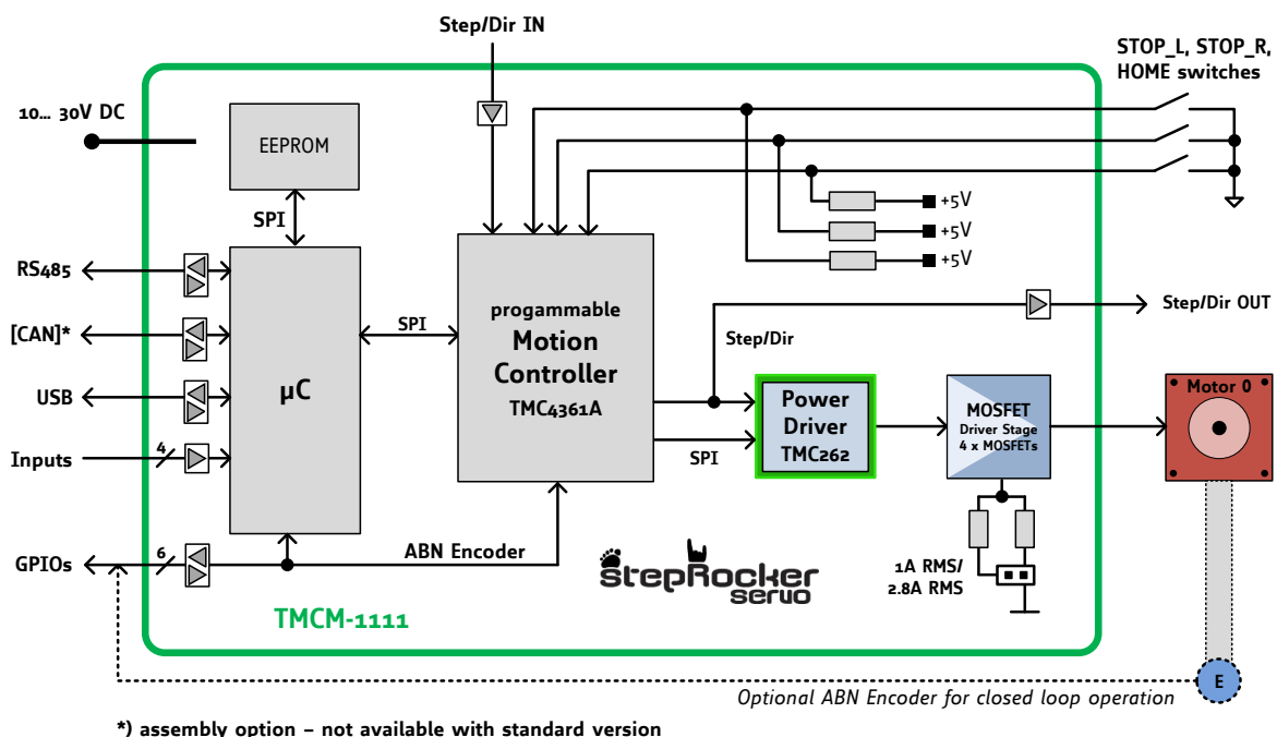
Figure 8: TMC1111 block diagram
