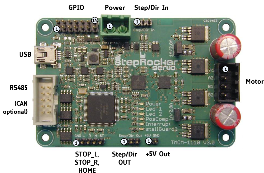
Figure 2: TMC-1111 stepRocker Connectors
