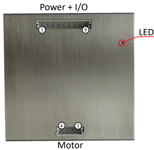
Figure 6: TMC-1076 connectors
