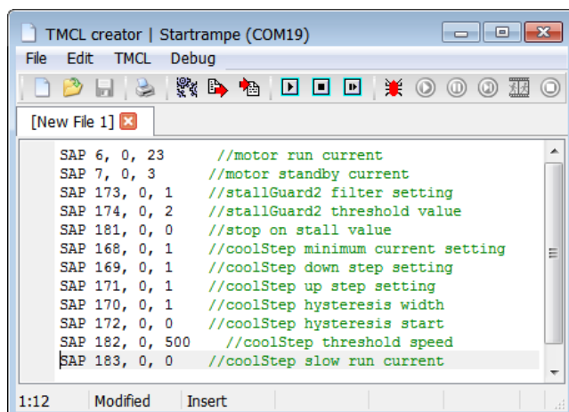
Figure 6.11 TMCL creator
