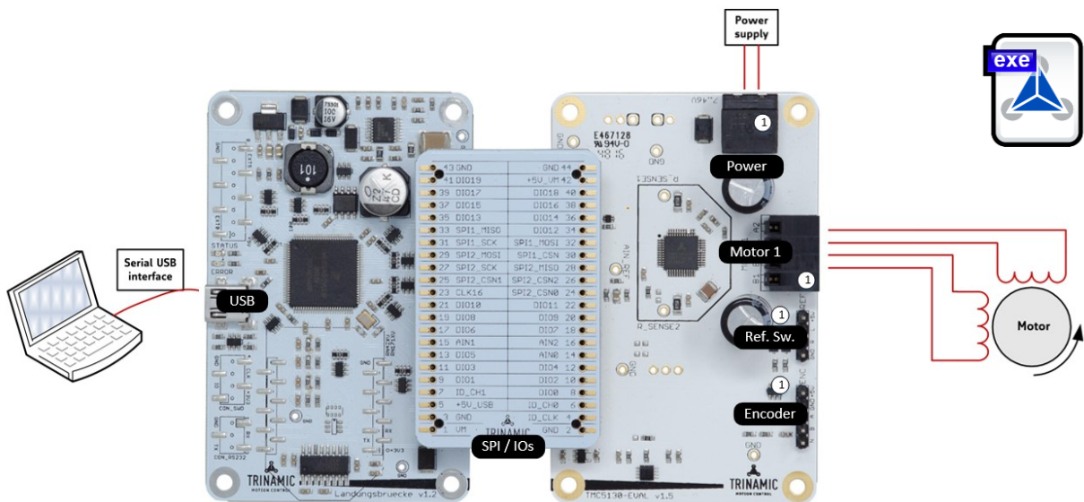
Figure 6.1 Getting started
