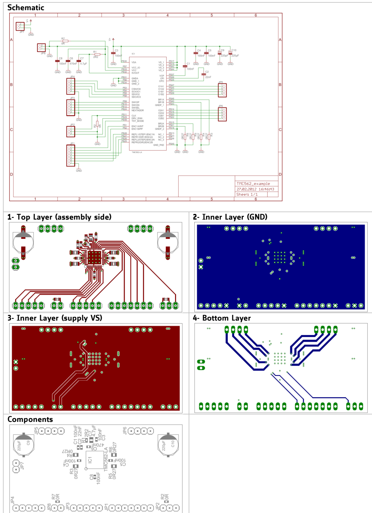
Figure 18.1 Layout example
