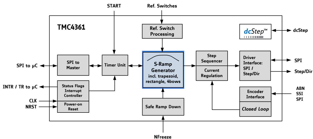
Figure 2: Block Diagram
