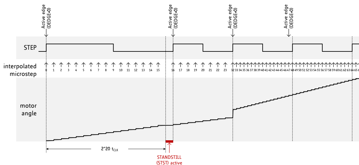
Figure 8.3 MicroPlyer microstep interpolation with rising STEP frequency.
