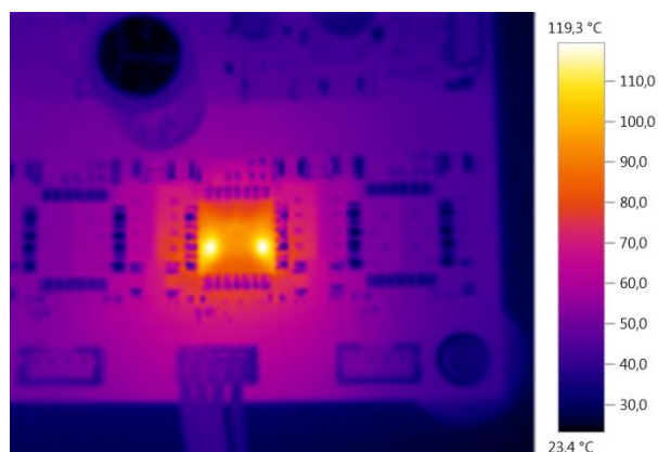
Figure 19.1 TMC2660 operating at 2.3A RMS (3.2A peak) on a 50cm 2 sized board
