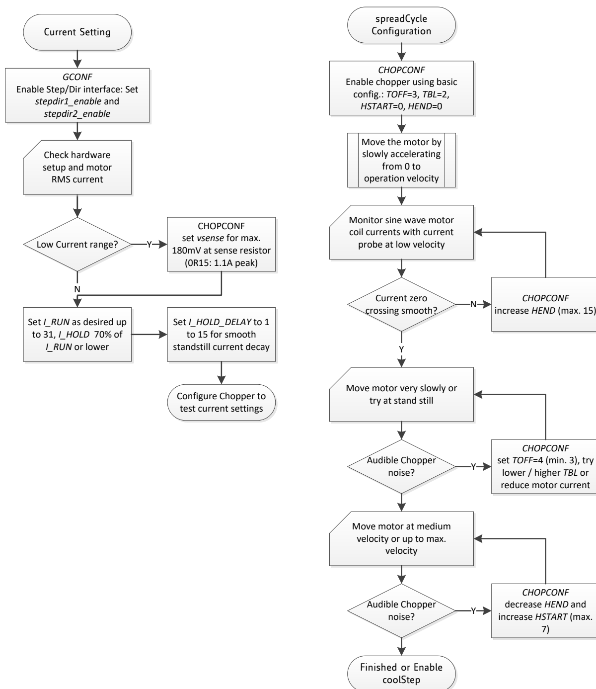
Figure 13.1 Current setting and configuration of spreadCycle
