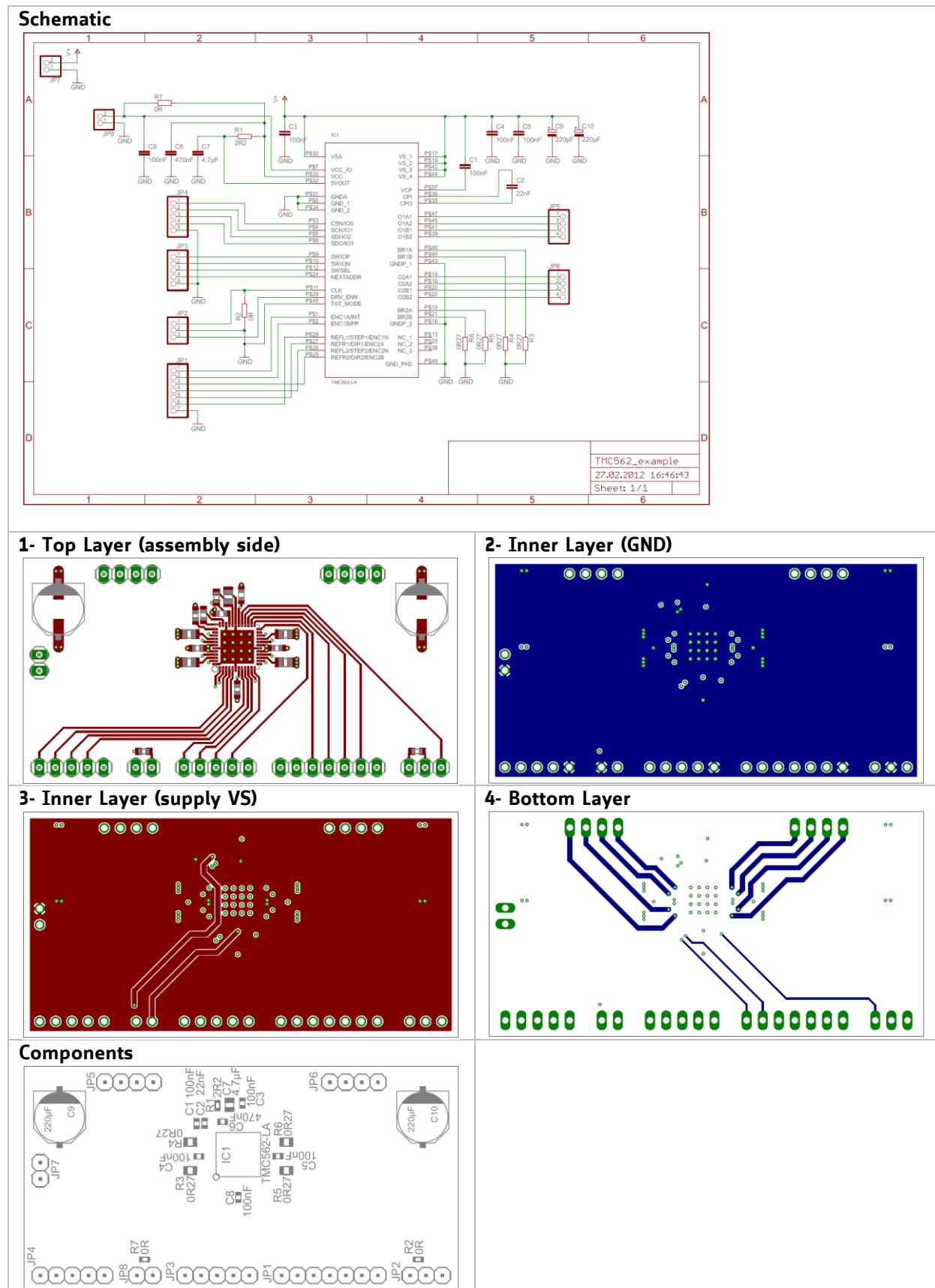
Figure 19.1 Layout example
