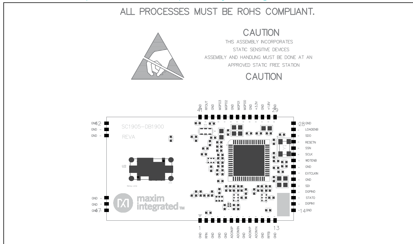
SC1905-DB1900—Assembly Drawing
