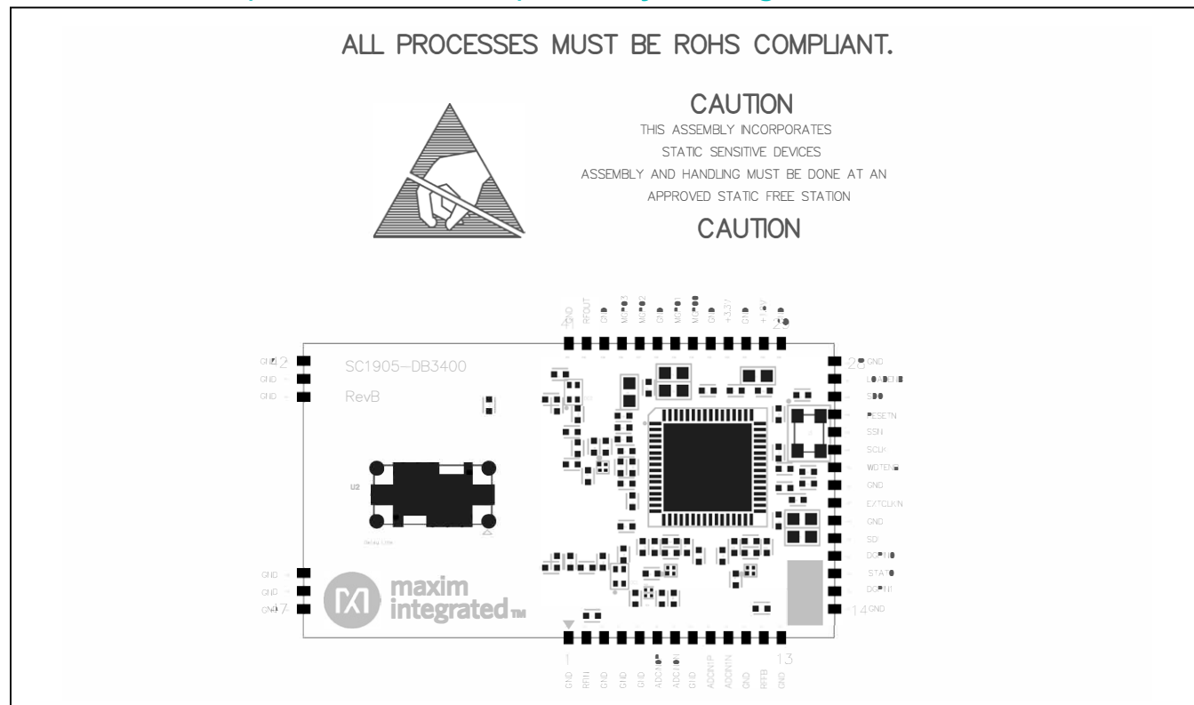
SC1905-DB3400—Assembly Drawing
