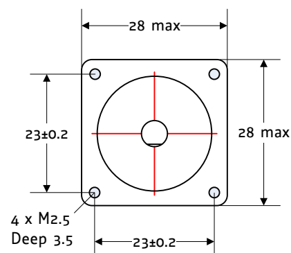
Figure 4.2: Dimensions (all values in mm)
