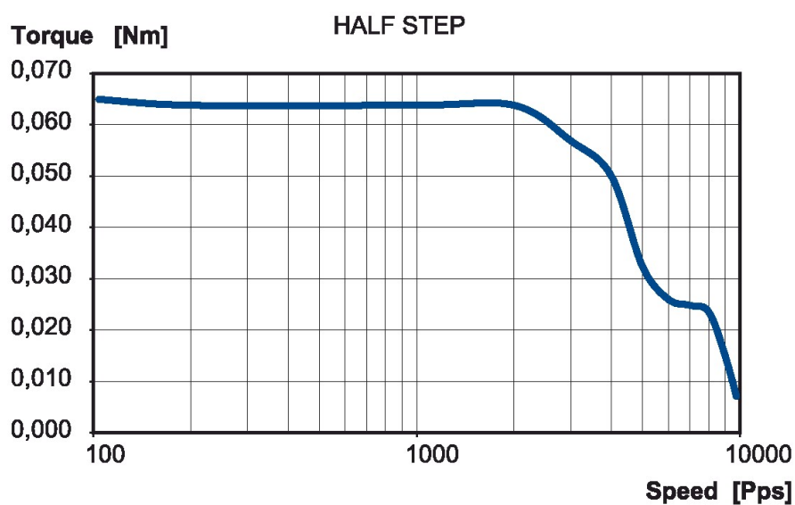
Figure 1: QSH2818-32-07-006 velocity vs. torque characteristic
