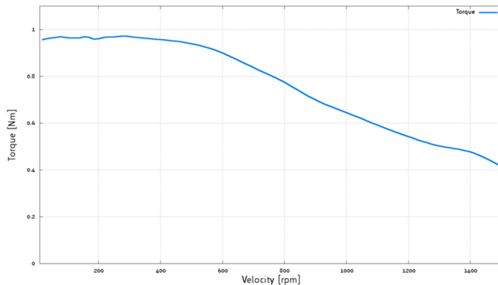
Figure 7: PD57-2-1378 torque vs. velocity 48V / 2.8A, 256 \mu steps
