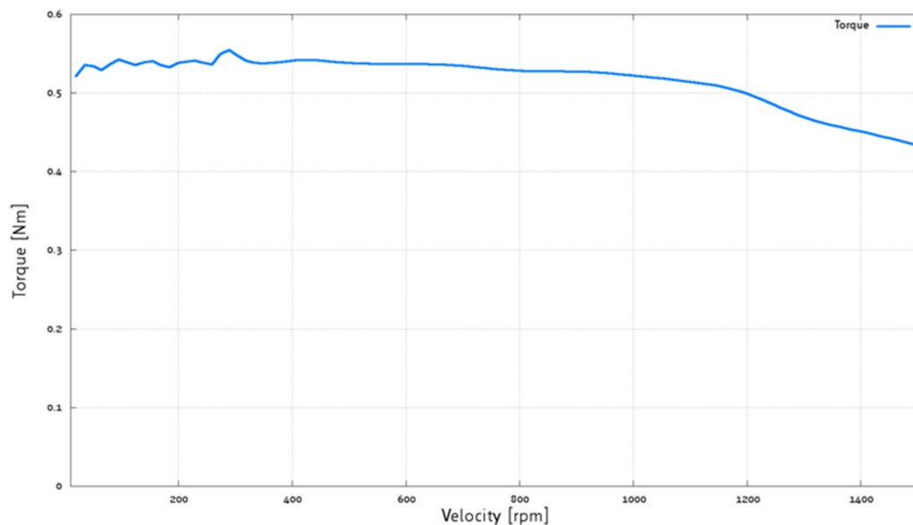
Figure 6: PD57-1-1378 torque vs. velocity 48V / 2.8A, 256 \mu steps
