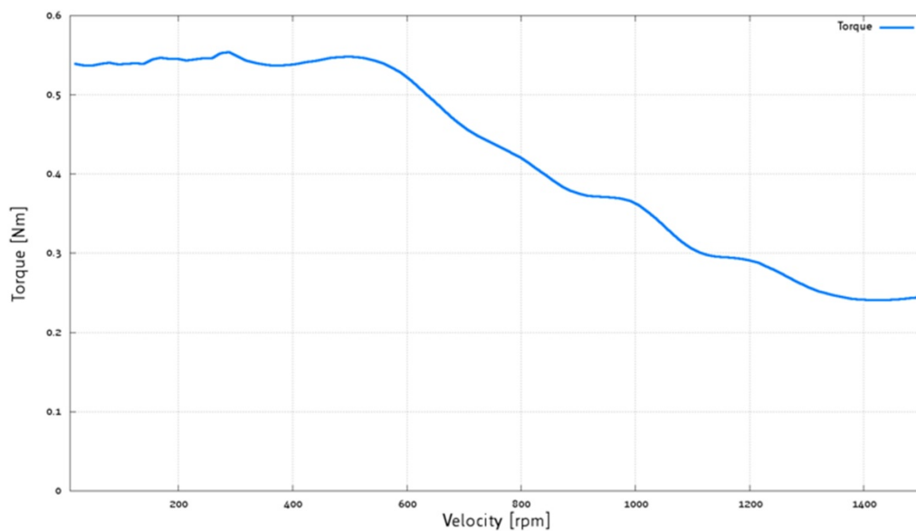
Figure 7: PD57-1-1276 torque vs. velocity 24V / 2.8A, 256 \mu steps
