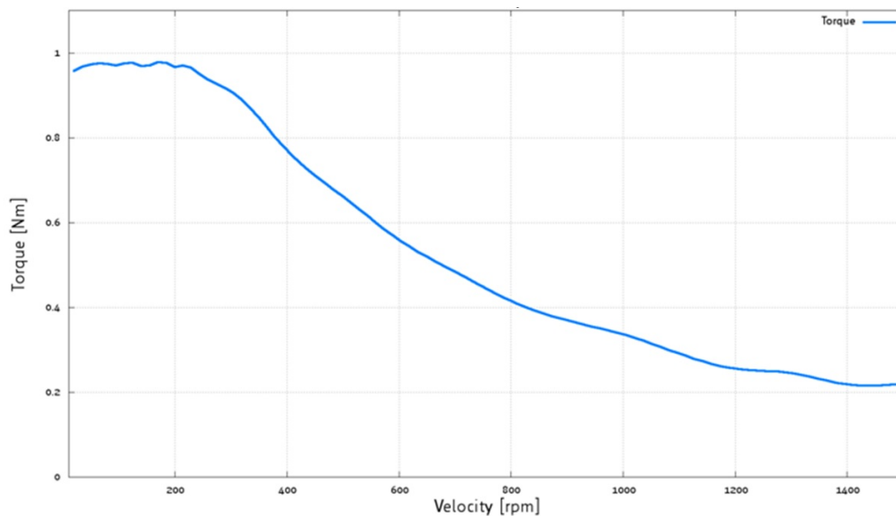
Figure 8: PD57-2-1276 torque vs. velocity 24V / 2.8A, 256 \mu steps
