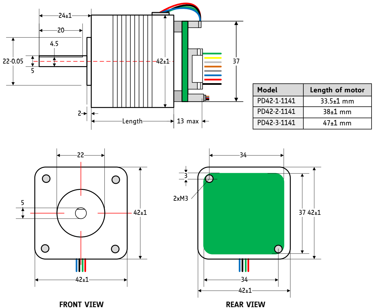
Figure 3.1 PD-1141 dimensions
